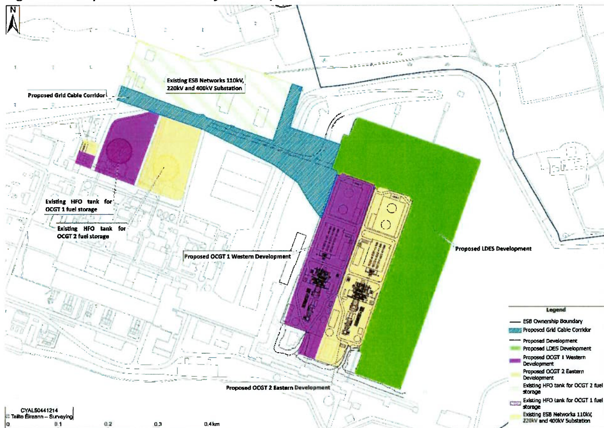
Figure 1.2: Proposed OCGT Site Layout – in pink
